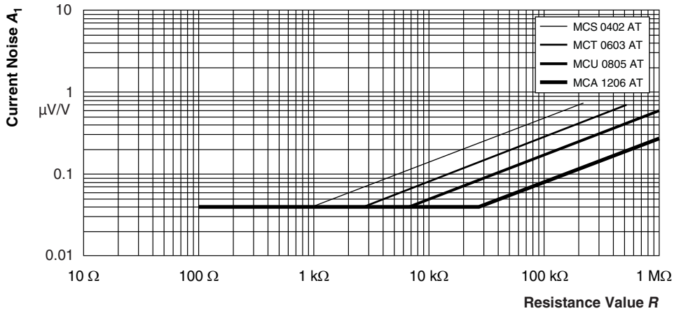
Current Noise
